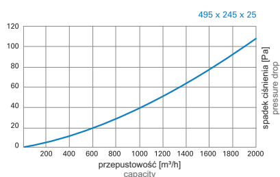
KP-FSI-495x245x25
