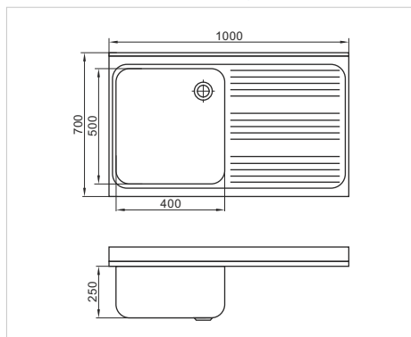
KZ-100705425/1L
