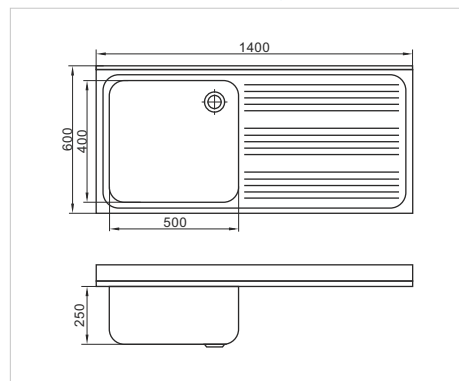
KZ-140605425/1L
