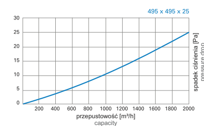
KP-FSI-495x495x25
